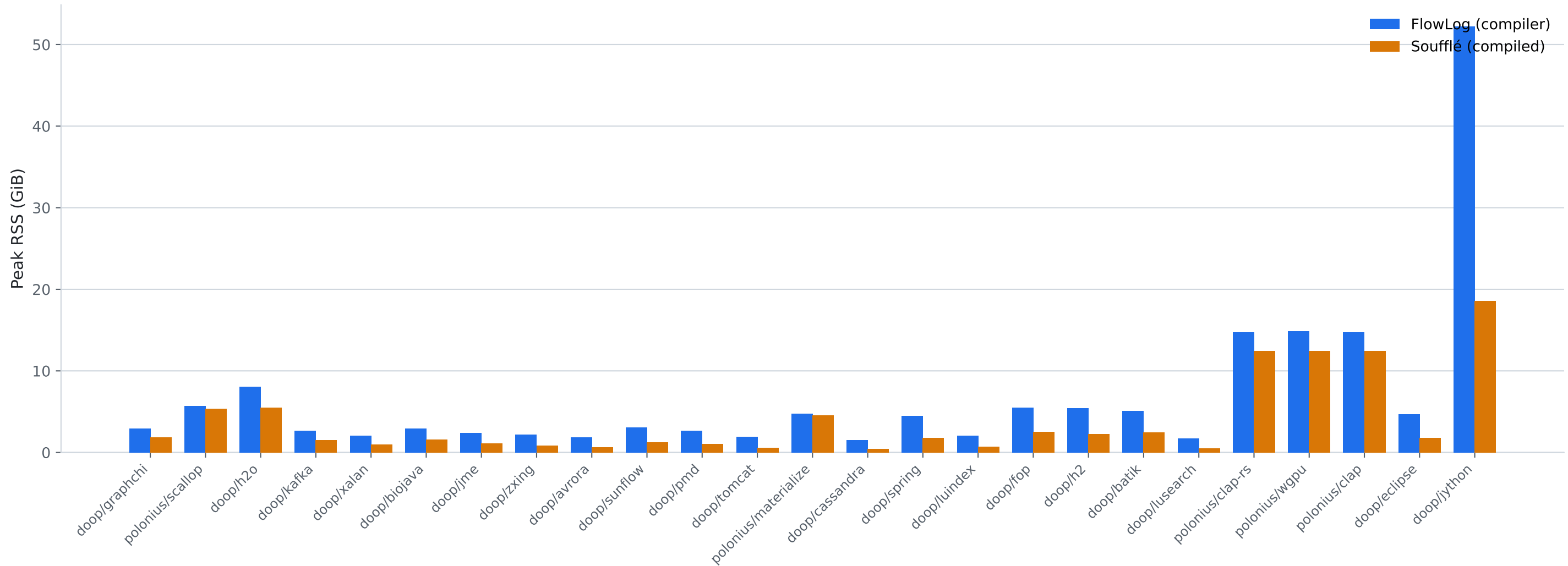
FlowLog vs Soufflé — peak memory · 25 workloads · lower is better
