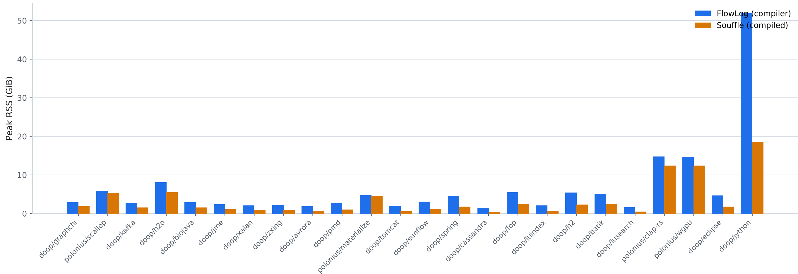
FlowLog vs Soufflé (DOOP + Polonius) — peak memory · 24 workloads · lower is better
