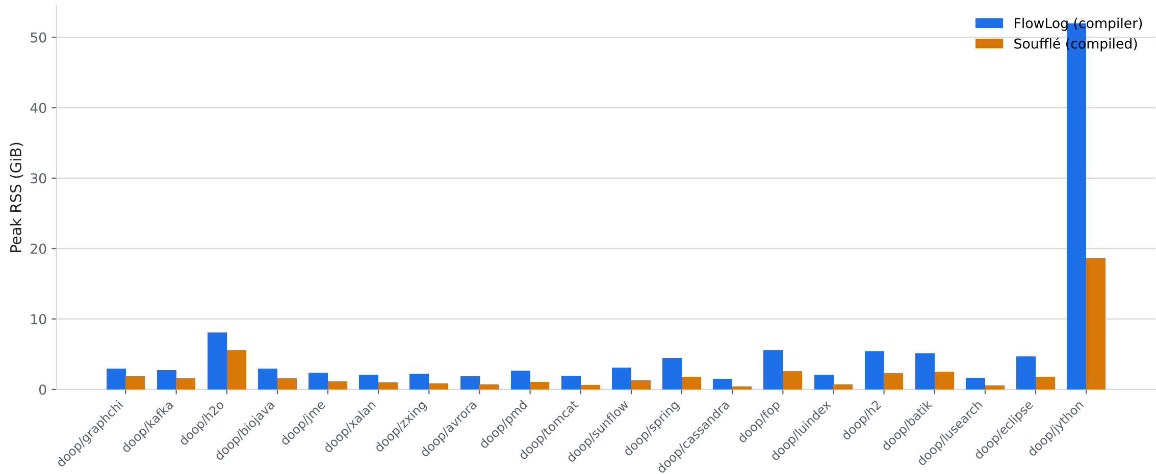
FlowLog vs Soufflé — DOOP — peak memory · 20 workloads · lower is better
