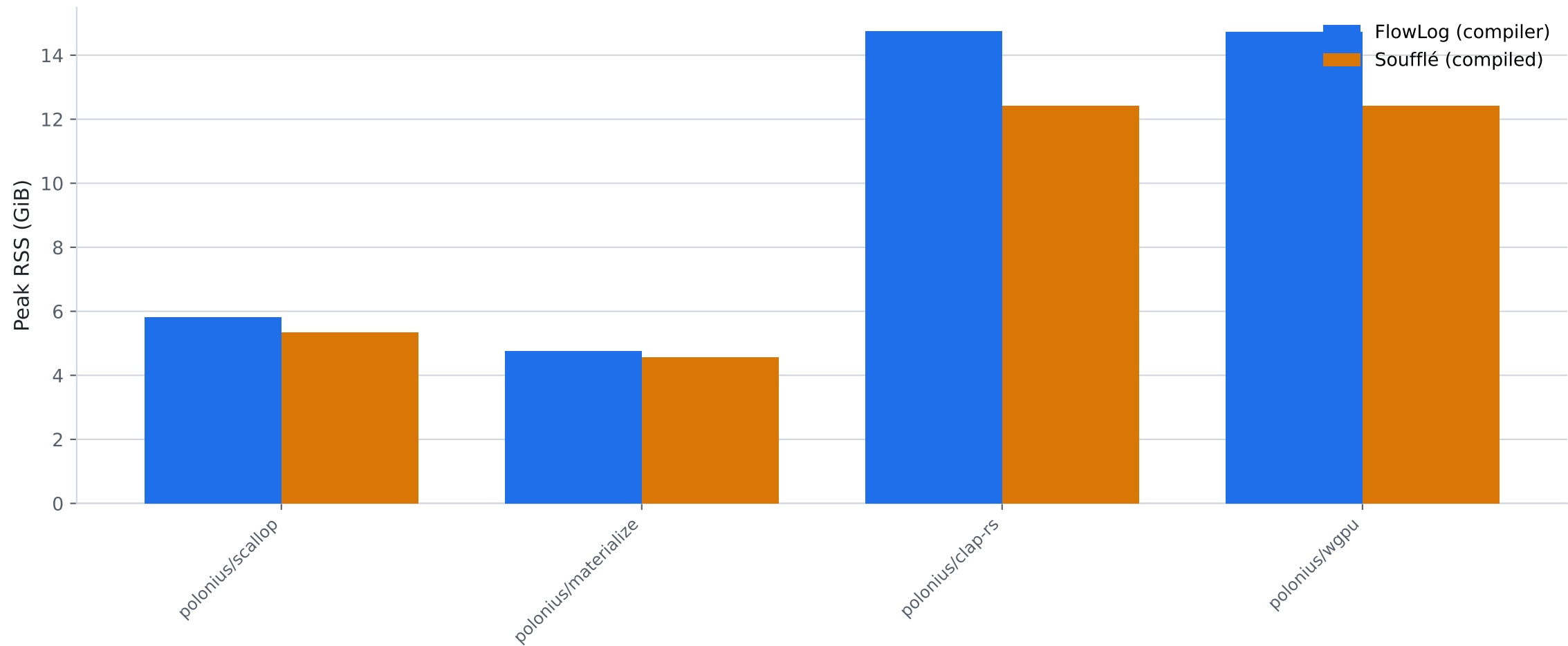
FlowLog vs Soufflé — Polonius — peak memory · 4 workloads · lower is better
