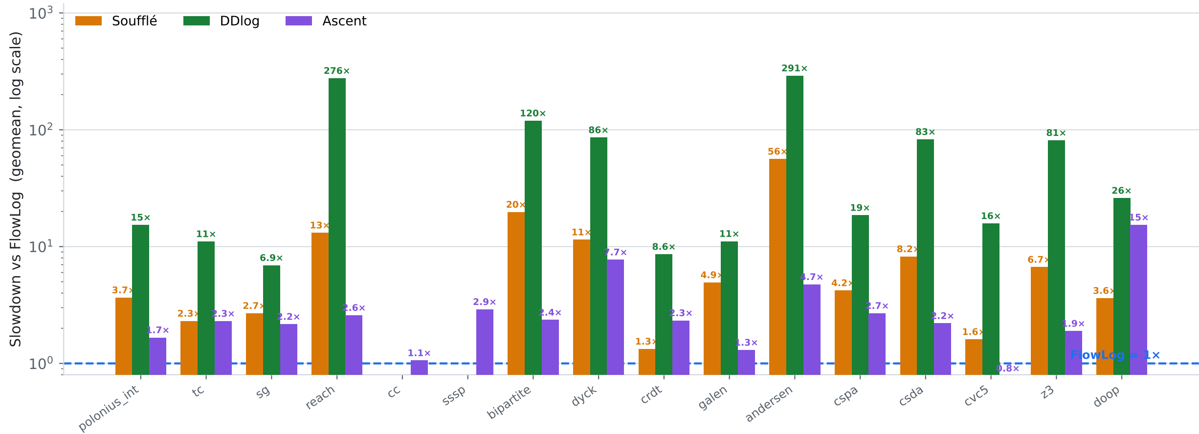
How much slower than FlowLog? Per-program geometric-mean slowdown (flowlog-west2, 4-engine sweep)
