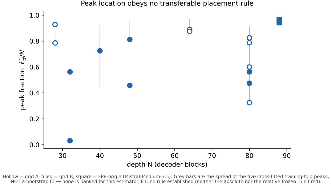
Figure 4: No placement rule established. Cross-fitted peak fraction \ell_{cf}^*/N against depth N . Hollow = grid A, filled = grid B, square = FP8-origin. Grey bars are the spread of the five cross-fitted training-fold peaks, not a bootstrap interval — none is banked for this estimator. Grid A and grid B are shown together for visual context only and are never pooled numerically.
