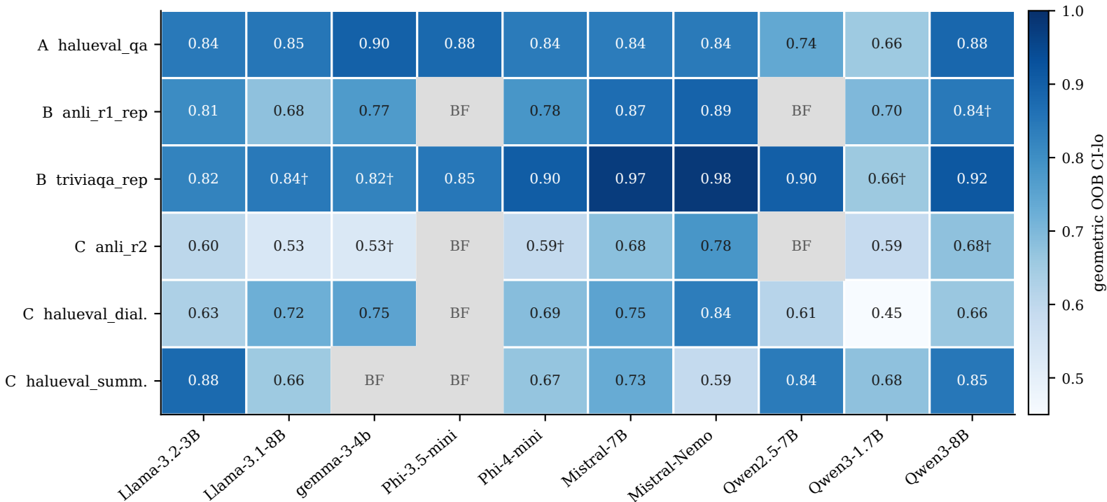
BENCH panel: registered-unit geometric OOB CI lower bound, 6 tasks × 10 models BF = behavioral-fail (no profile); † = commitment-fail (geometry shown, cannot count toward a bar)
