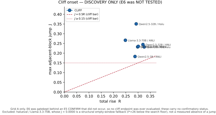
Figure 3: Cliff onset — DISCOVERY ONLY. Grid A cells: largest adjacent-block jump J against total rise R , with the two registered cliff bars drawn. E6 was gatekept behind an E5 CONFIRM that did not occur, so no cliff endpoint was ever evaluated and these points carry no confirmatory status. Llama-3.3-70B/haluval_qa is excluded: its J = 0.0000 is a structural empty-window fallback, not a measured zero.
