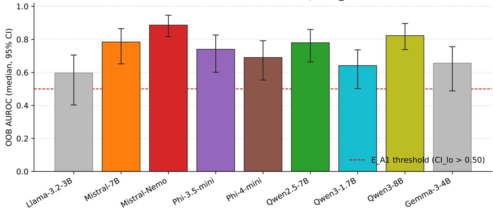
ACE on ANLI R1 (n=200): 7/9 pass E_A1
