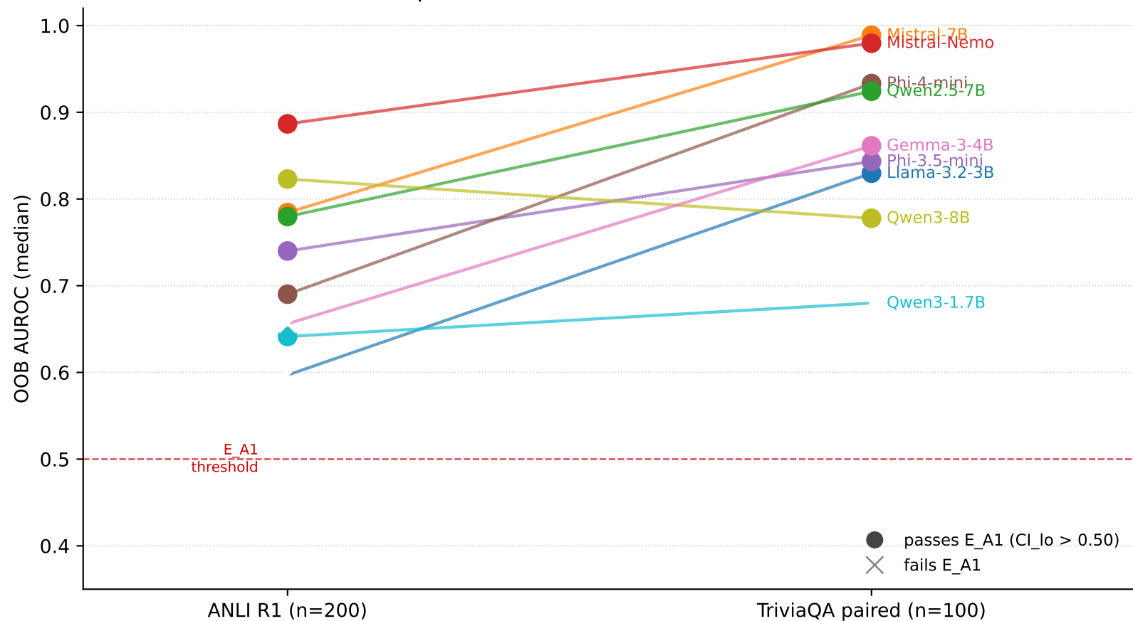
ACE per-model AUROC: ANLI R1 → TriviaQA
