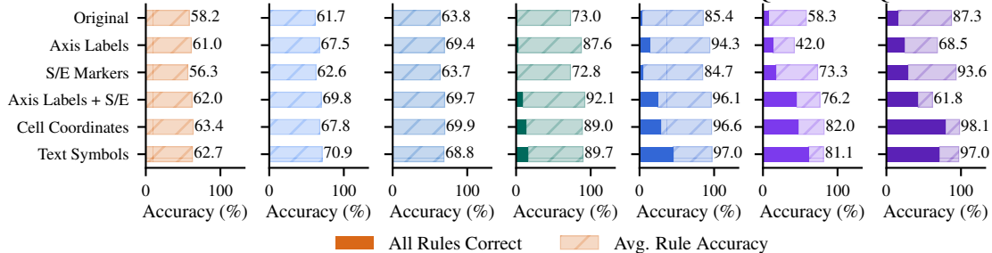
Mistral Small 3.2
