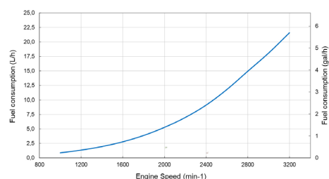
4JH110 Fuel consumption (propload exp 3.0)
