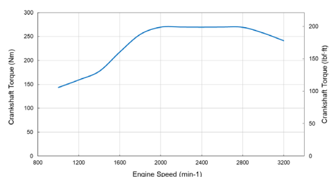
4JH110 Torque curve
