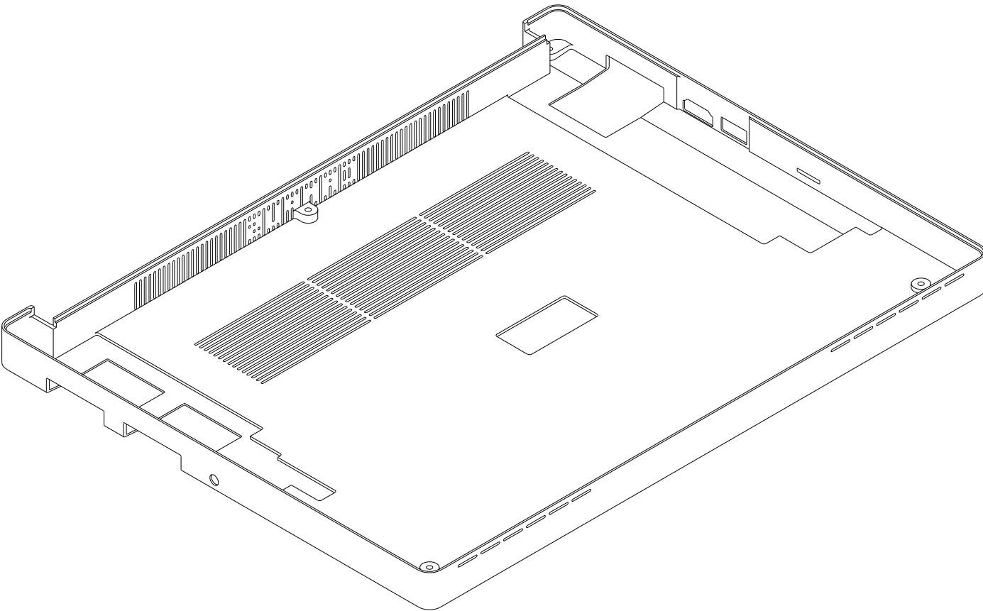
ISOMETRIC VIEW
