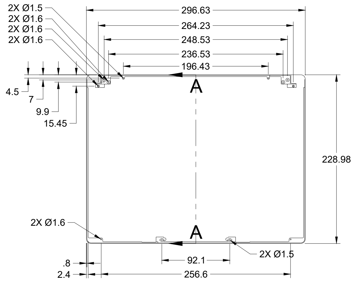
BOTTOM VIEW
