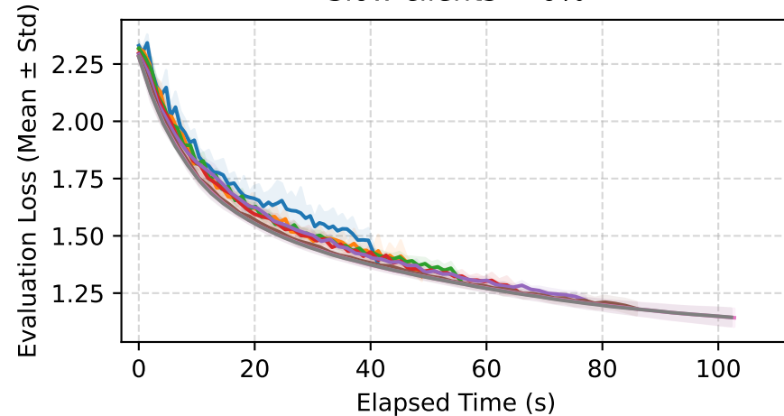
Slow clients = 0%
