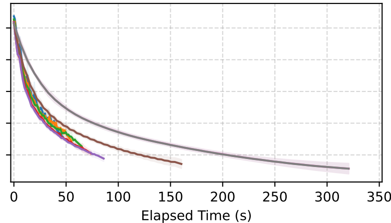
Slow clients = 20%
