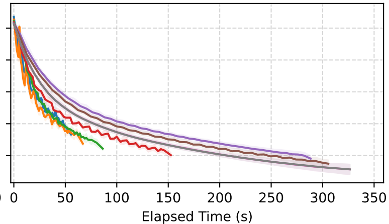
Slow clients = 50%
