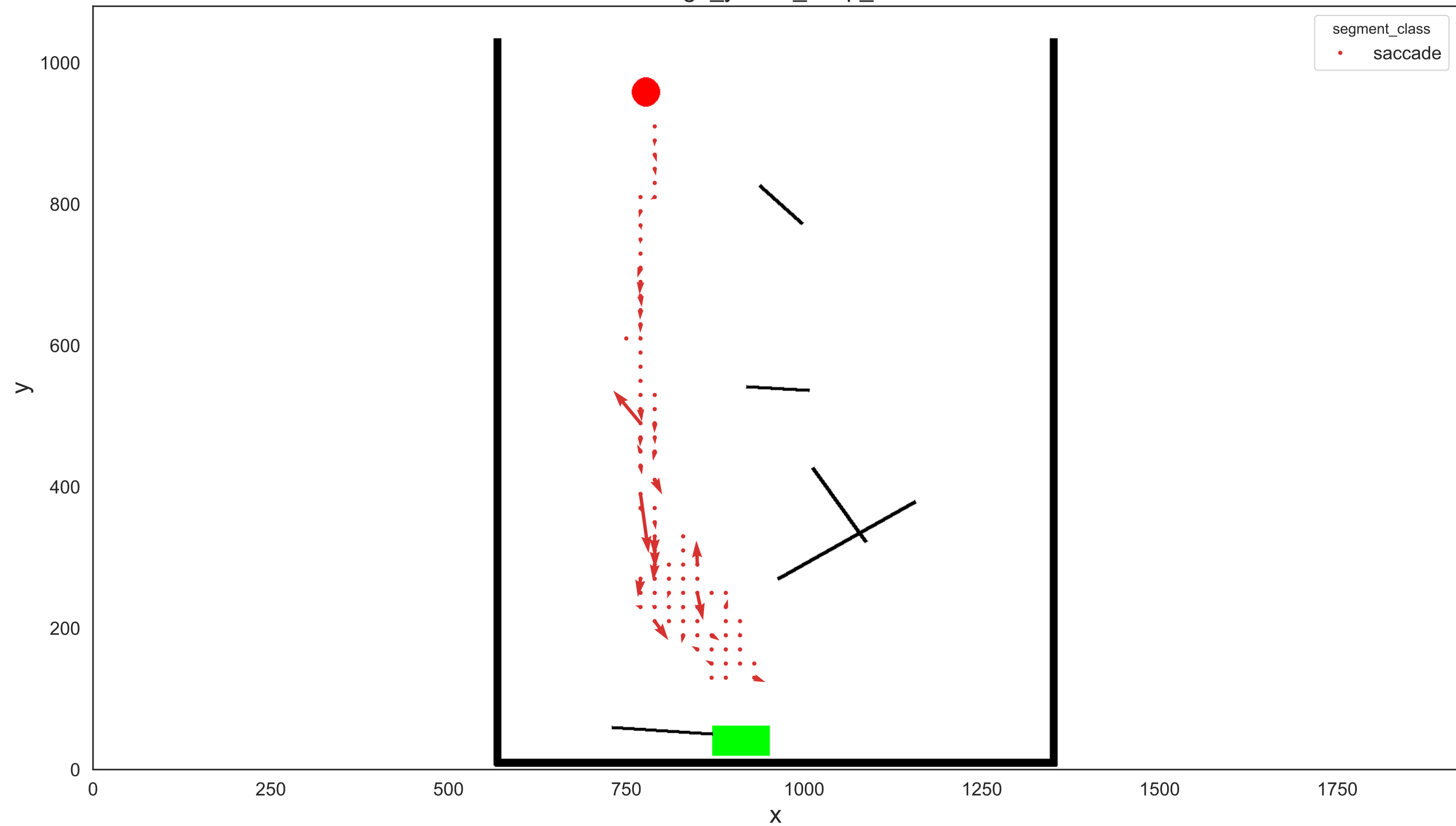
high_yescol_nosp_3
