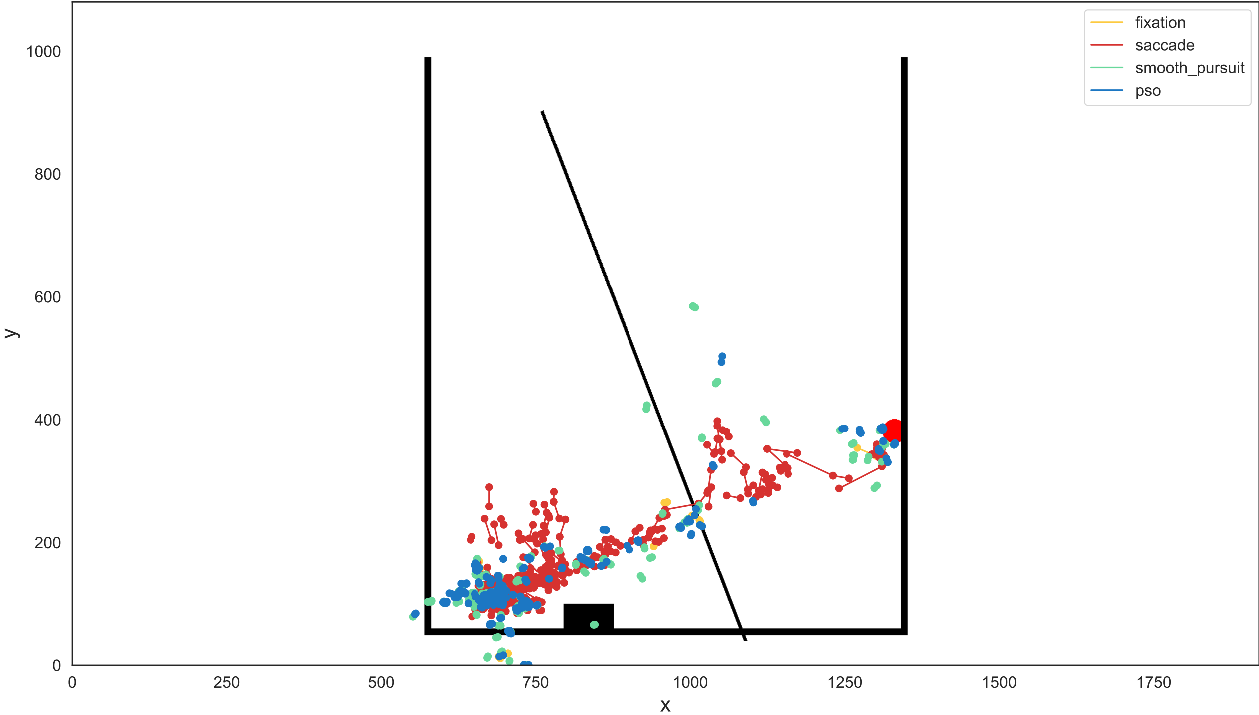
Scene: high_nocol_yessp_1
