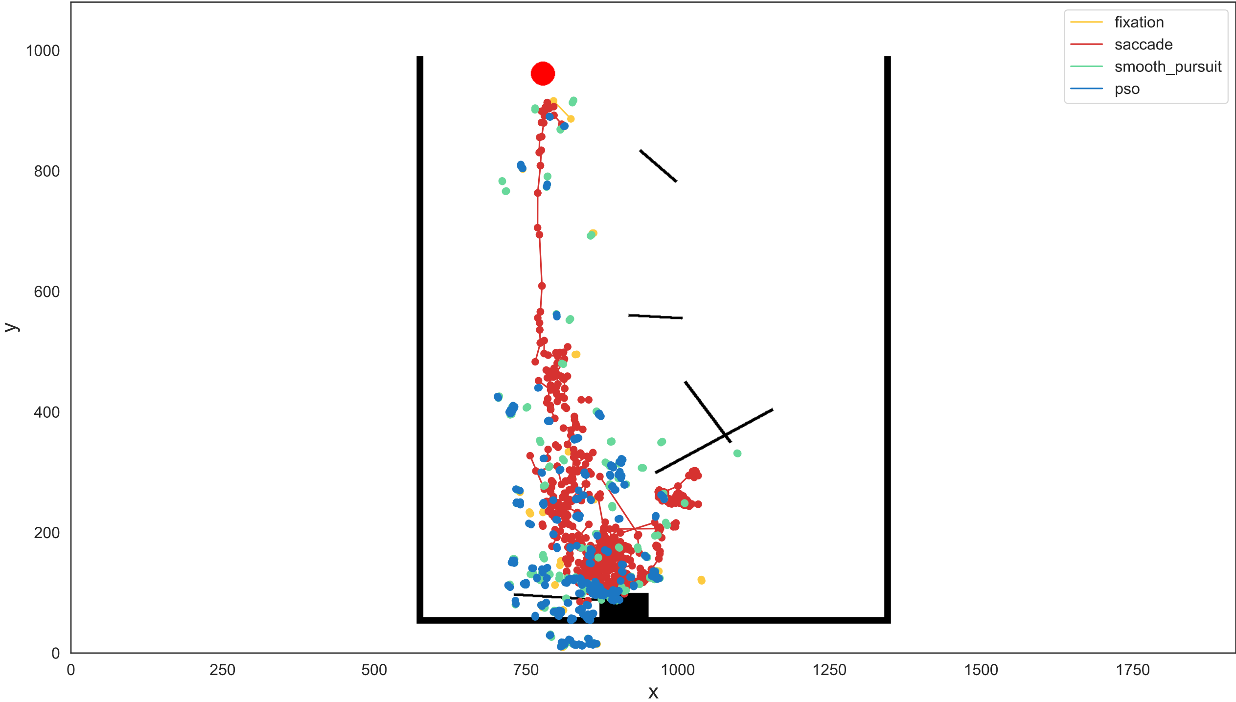
Scene: high_yescol_nosp_3
