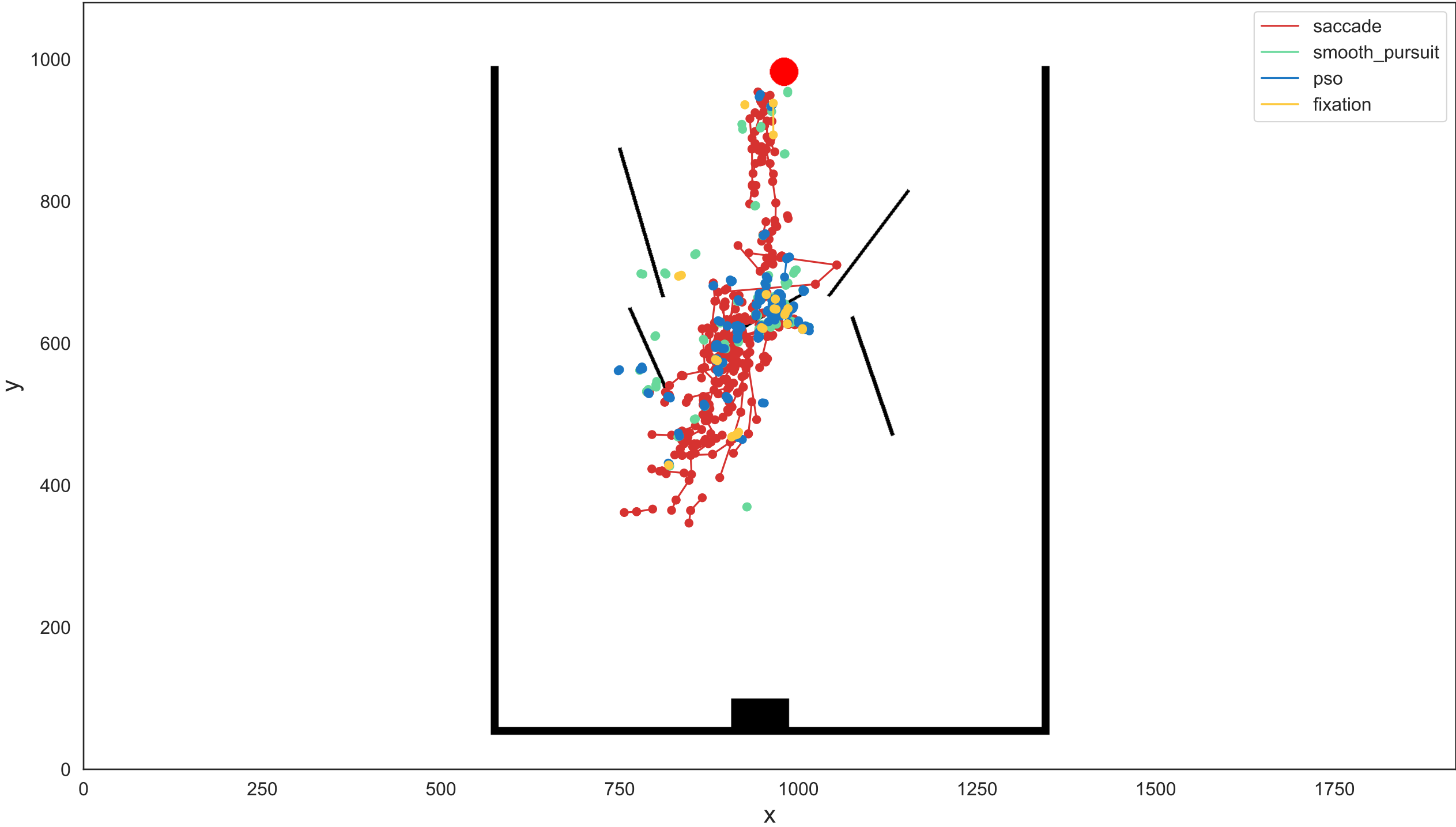
Scene: high_yescol_nosp_4
