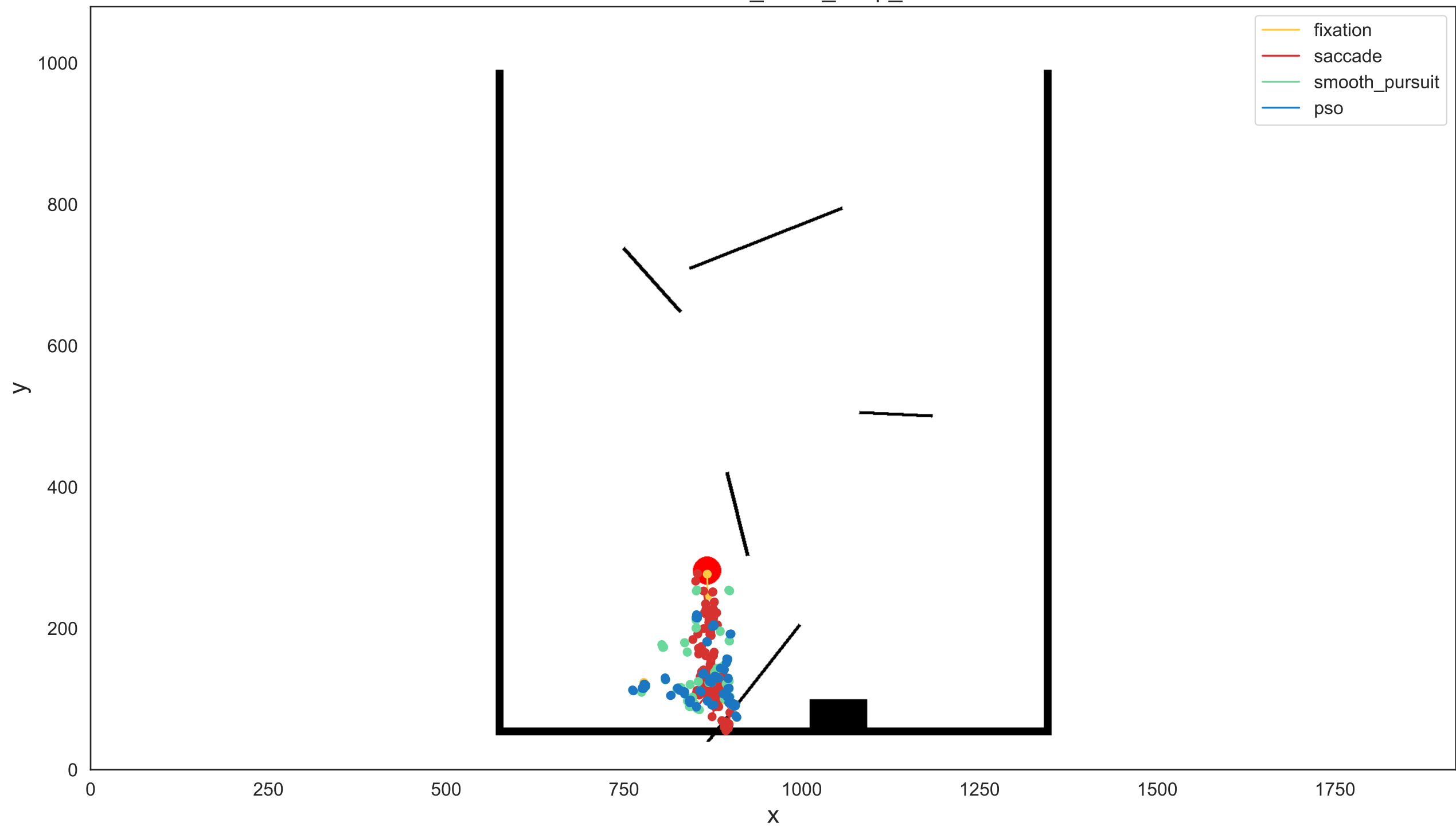
Scene: low_nocol_nosp_3
