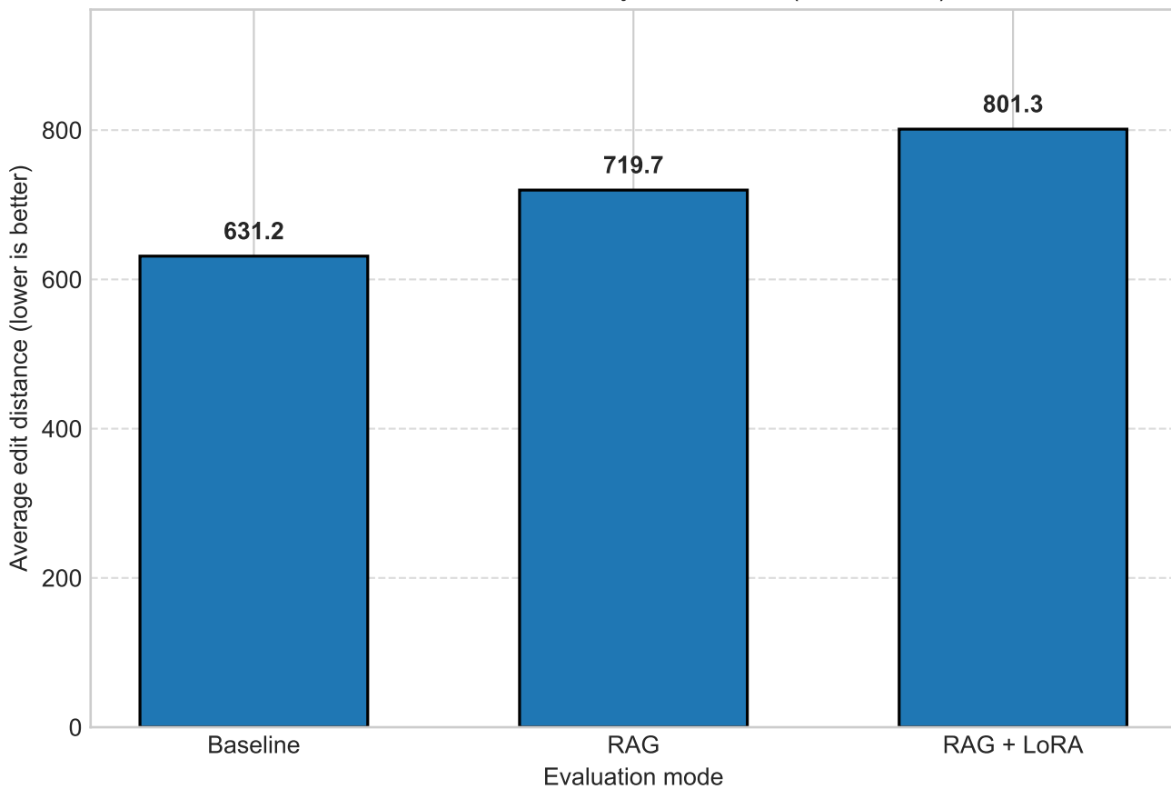
FIM Edit Distance – TinyLlama 1.1B (Fine-tuned)
