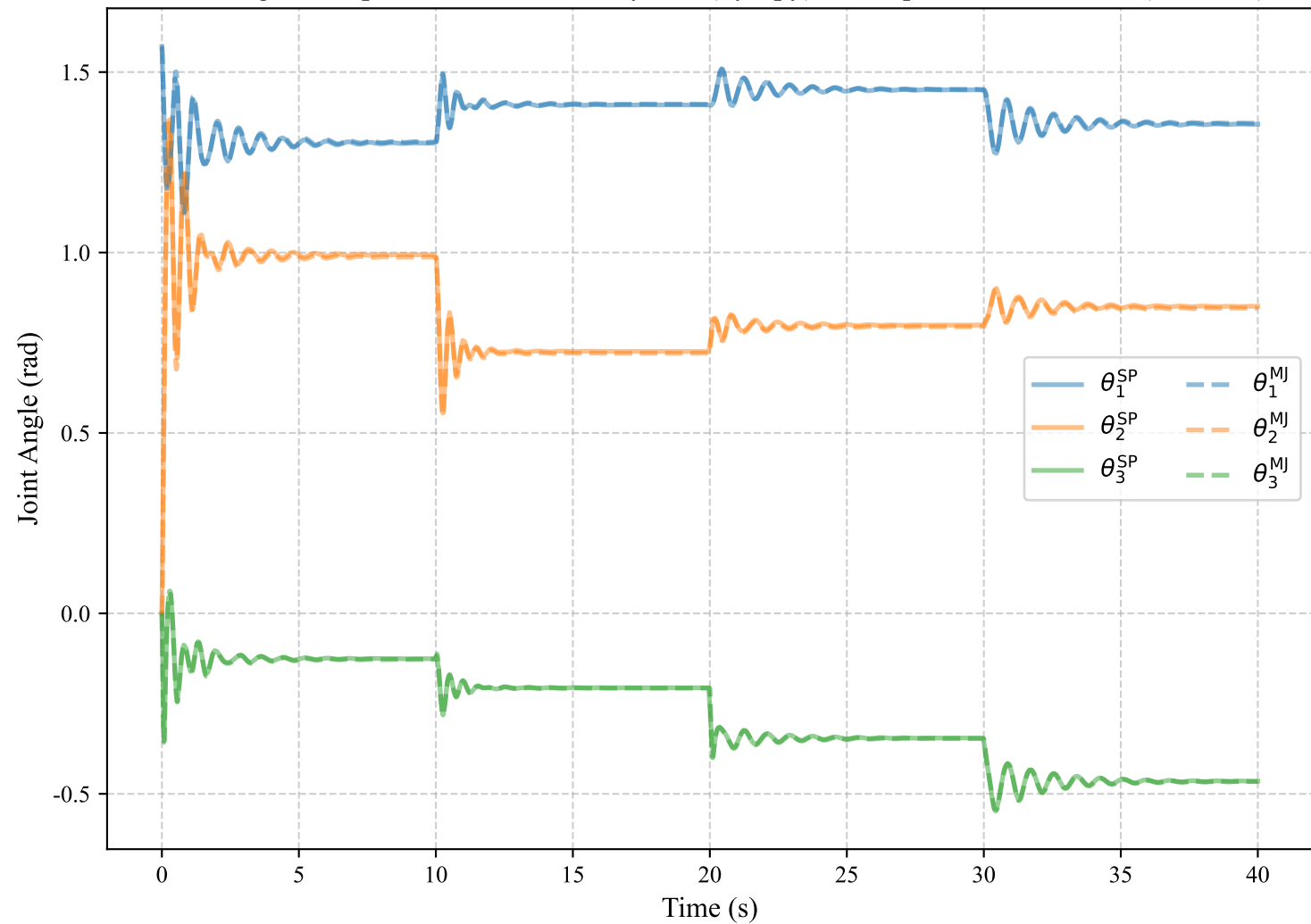
Joint Angle Comparison between Analytical (SymPy) and EquiMus Simulation (MuJoCo)
