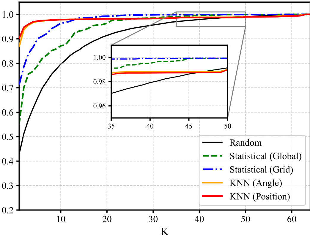
Normalized Spectral Efficiency
