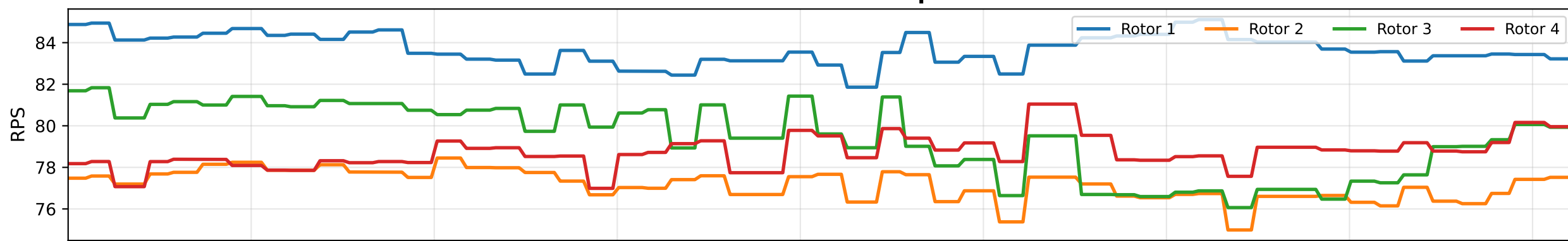
Ground Truth Motor Speeds
