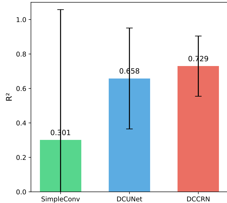
Coefficient of Determination (Higher is Better)
