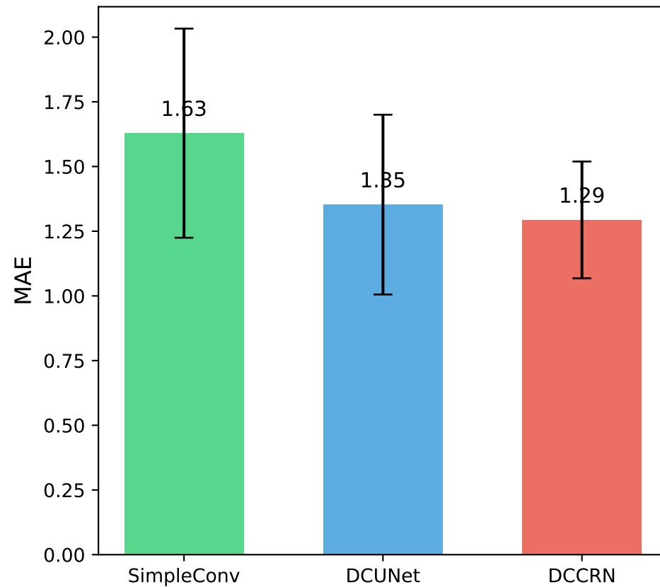
Mean Absolute Error (Lower is Better)
