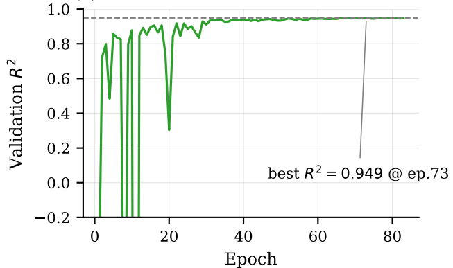
(b) Validation coefficient of determination
