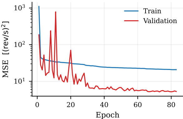
(a) Training and validation MSE
