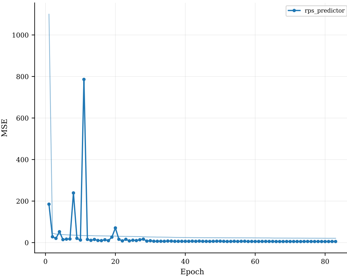
Training / Validation MSE
