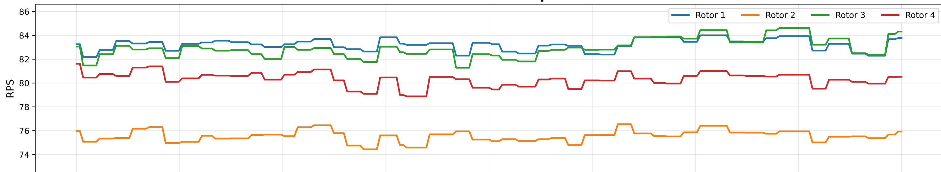
SimpleConv Prediction (MAE=1.23) — Full=Prediction, Dotted=Target
