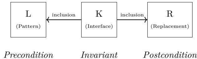
Figure 3.1: The DPO span: The fundamental atom of rewriting physics.
