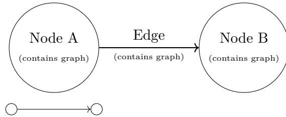
Figure 2.1: Visualizing an RMG: Nodes and edges are containers for deeper structure.
