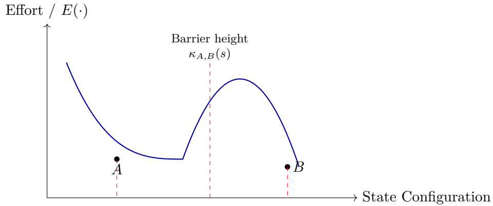
Figure 5.7: A schematic energy landscape: two basins A and B separated by a high-curvature barrier. The barrier height reflects the minimal additional effort required to transition between basins.
