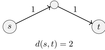
Figure 5.5: Two parallel notions of Rulial Distance. Left: Each rewrite has unit cost, so distance counts the number of steps. Right: Each rewrite has a Lagrangian cost, producing the weighted distance used for optimization in Chapter 18. Chapter 18 generalizes the metric of Chapter 5 by replacing unit weights with resource-aware costs.
