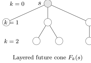
Figure 5.6: A schematic future cone rooted at s , stratified by Rulial Distance. Each layer represents states exactly k rewrites away.
