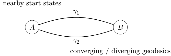
Figure 33.4: Heuristic depiction of curvature in MRMW: nearby geodesics between similar states either converge (positive curvature) or diverge (negative curvature).
