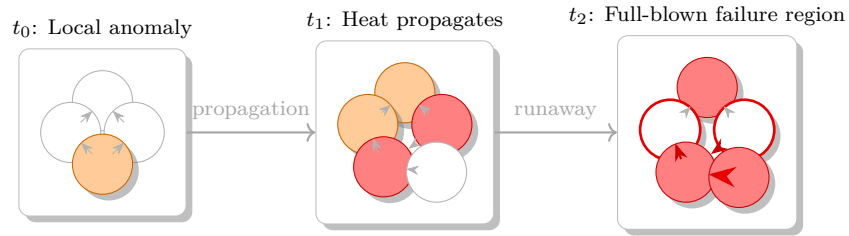
Figure 5.8: Temporal evolution of Rulial Heat. A small local deviation at t_0 becomes a structurally significant divergence at t_1 , and by t_2 the bug has carved out an entire hot region in the universe. Debugging is the act of locating and cooling this region.
