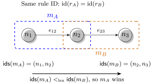
Figure 5.2: Deterministic tie-breaking: two competing matches of the same rule. Canonical ID ordering selects m_A as the unique next rewrite.
