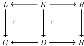
Figure 3.4: The Double-Pushout diagram. The rewrite flows from G to H through the intermediate context D . The two marked squares are the “make the hole” step, and the “fill the hole” step.
