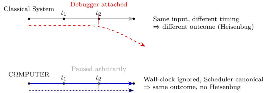
Figure 5.9: In classical systems, attaching a debugger perturbs timing and can change the outcome (a Heisenbug). In COMPUTER , the Scheduler ignores time, so observation cannot alter the worldline. The Observer Effect is dead.
