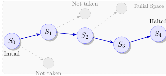
Figure 5.1: A worldline is the actual path taken through Rulial Space. Ghost paths represent possible futures that were never chosen. The Scheduler collapses this cloud of possibility into a single deterministic sequence.
