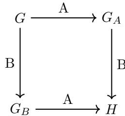
Figure 3.6: When two rules act on disjoint regions, their steps commute: either order lands in the same universe H . This is DPO’s “parallelism without races.”
