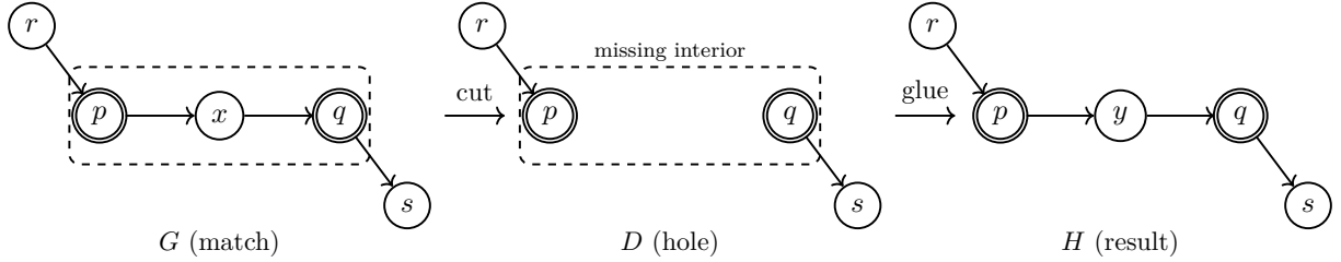
Figure 3.3: A cut-and-glue view of one DPO step. The dashed box marks the matched region. The double-bordered nodes are the interface: they stay. The cut removes the interior. The glue installs a replacement interior along the same boundary.
