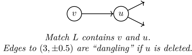
Figure 3.5: A visualization of the dangling condition. If the rule attempts to delete u , it must also account for all incident edges, or the rewrite is rejected.
