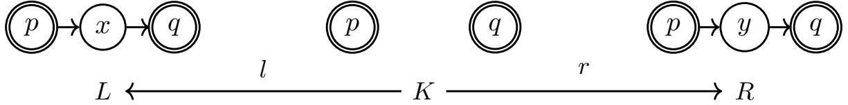
Figure 3.2: A concrete DPO rule. The interface K (double-bordered nodes) must survive the rewrite. Everything in L outside of K is removed; everything in R outside of K is added.
