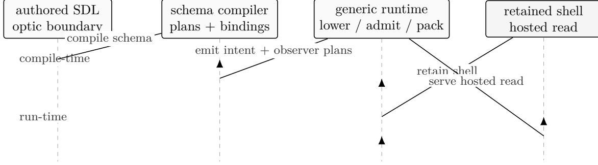
Figure 4: Authored optic boundaries compile into generic admission and observer machinery.
