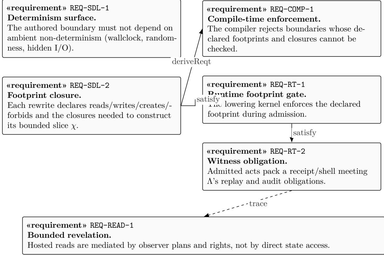
Figure 5: A requirement view of the compiler seam: authored boundaries are constrained so that admission remains deterministic, checkable, and witness-bearing.
