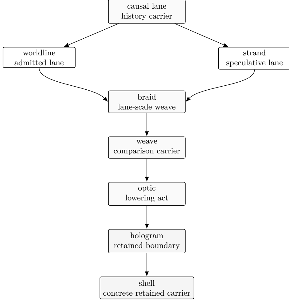
Figure 1: Nouns and roles. Lanes carry history; worldlines and strands are admitted and speculative lane forms. A braid is the lane-scale special case of a weave. The optic lowers a weave over a bounded site, the hologram names the retained boundary of that act, and the shell is its concrete carrier.
