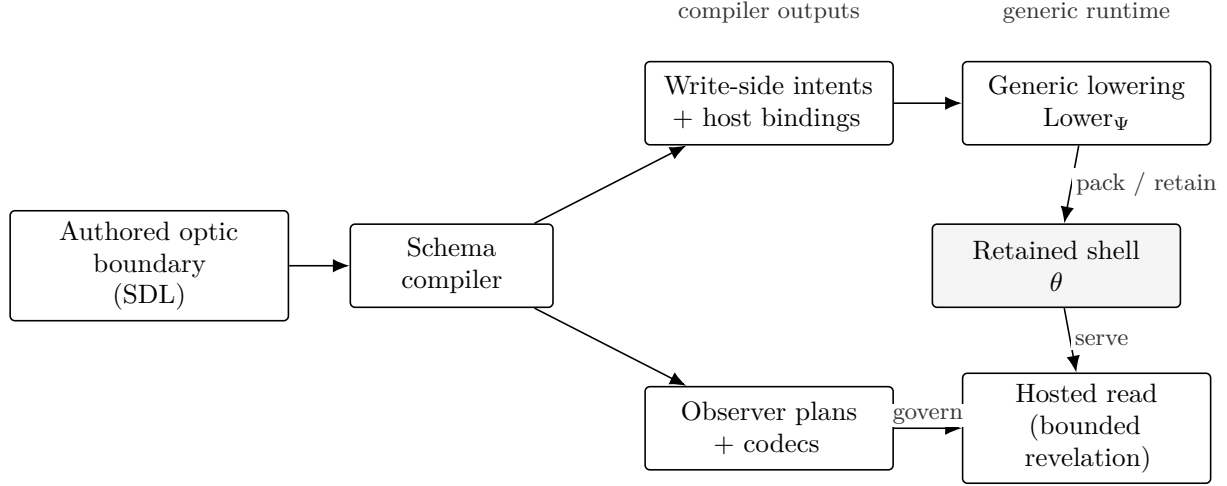
Figure 4: Authored optic boundaries compile into two runtime-facing artefacts. Write-side intents drive generic lowering. Read-side observer plans govern bounded revelation over the retained shell.
