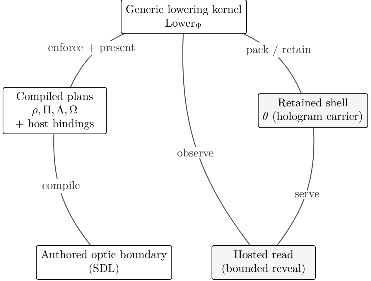
Figure 4: Authored optic boundaries compile into generic admission and observer machinery.
