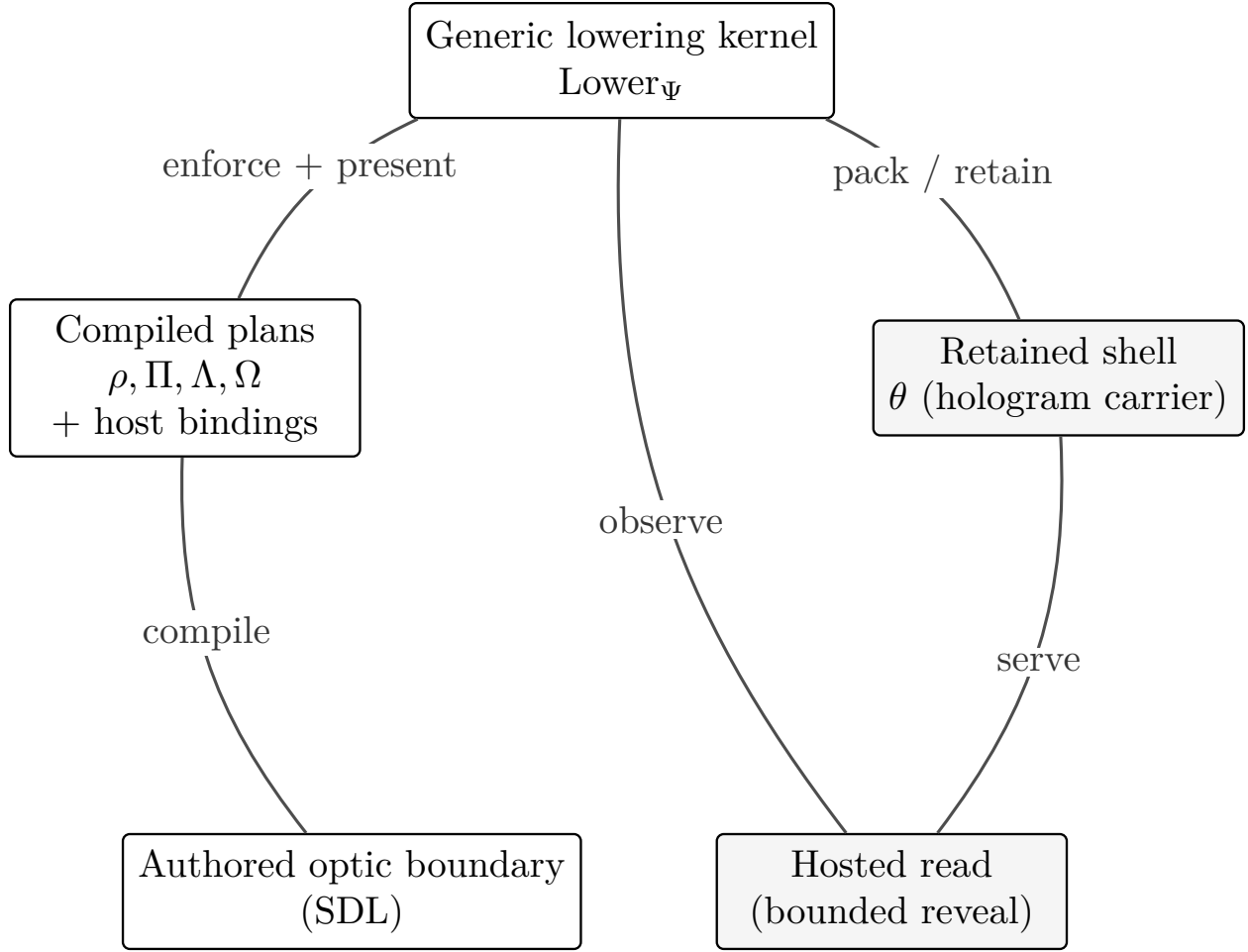
Figure 4: Authored optic boundaries compile into generic admission and observer machinery.
