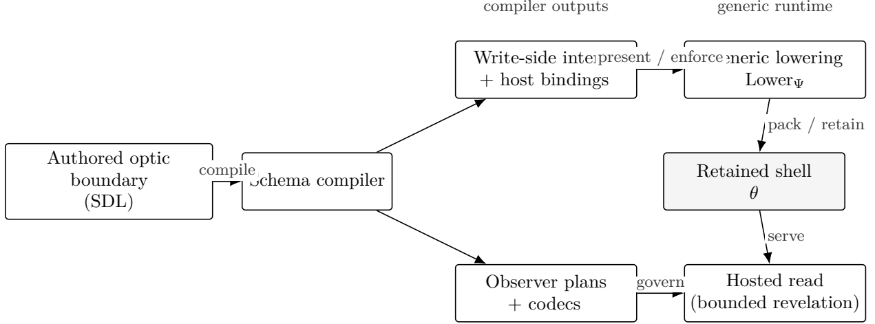
Figure 4: Authored optic boundaries compile into two runtime-facing artefacts. Write-side intents drive generic lowering. Read-side observer plans govern bounded revelation over the retained shell.
