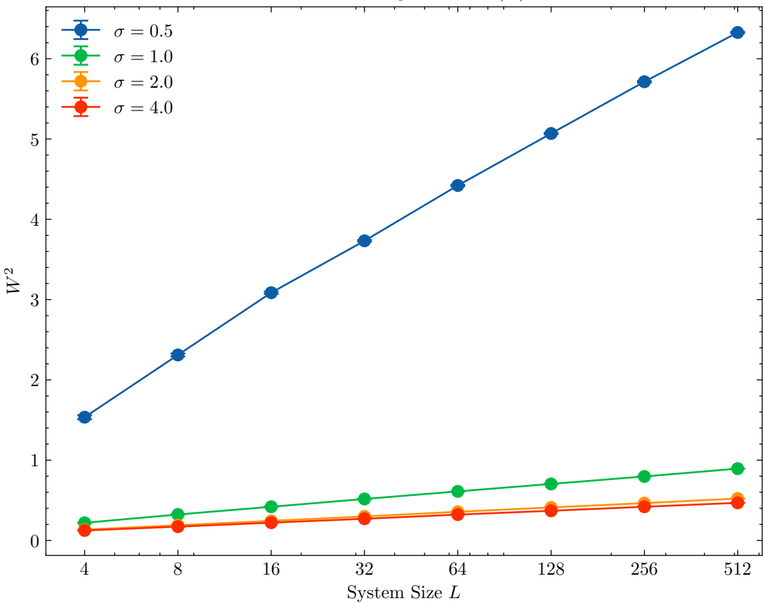
Surface Roughness W^2(L)
