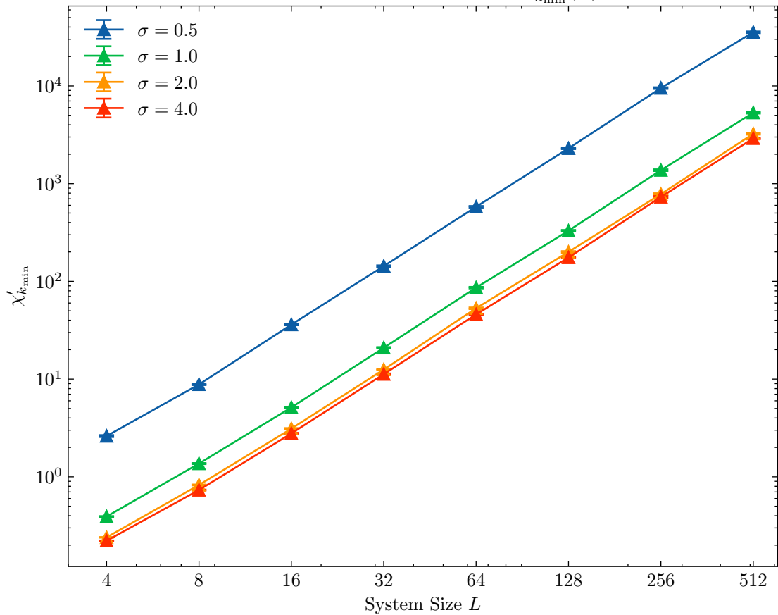
Connected Structure Factor \chi'_{k_{\min}}(L)
