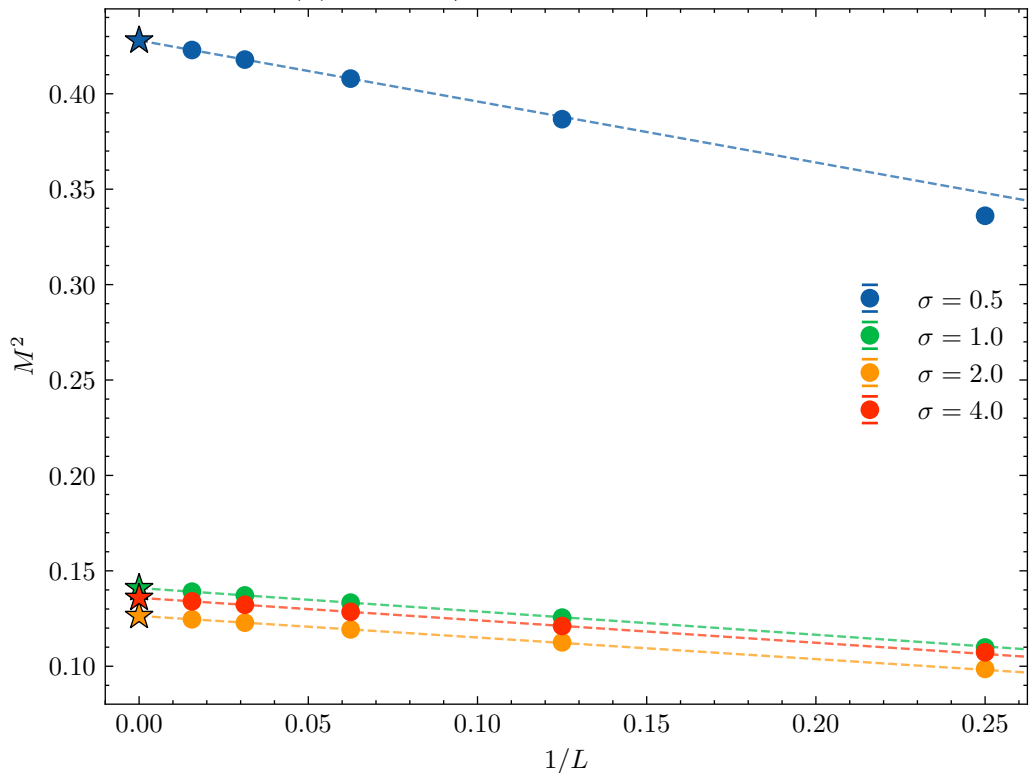
(b) M^2 vs 1/L , extrapolation to L \rightarrow \infty
