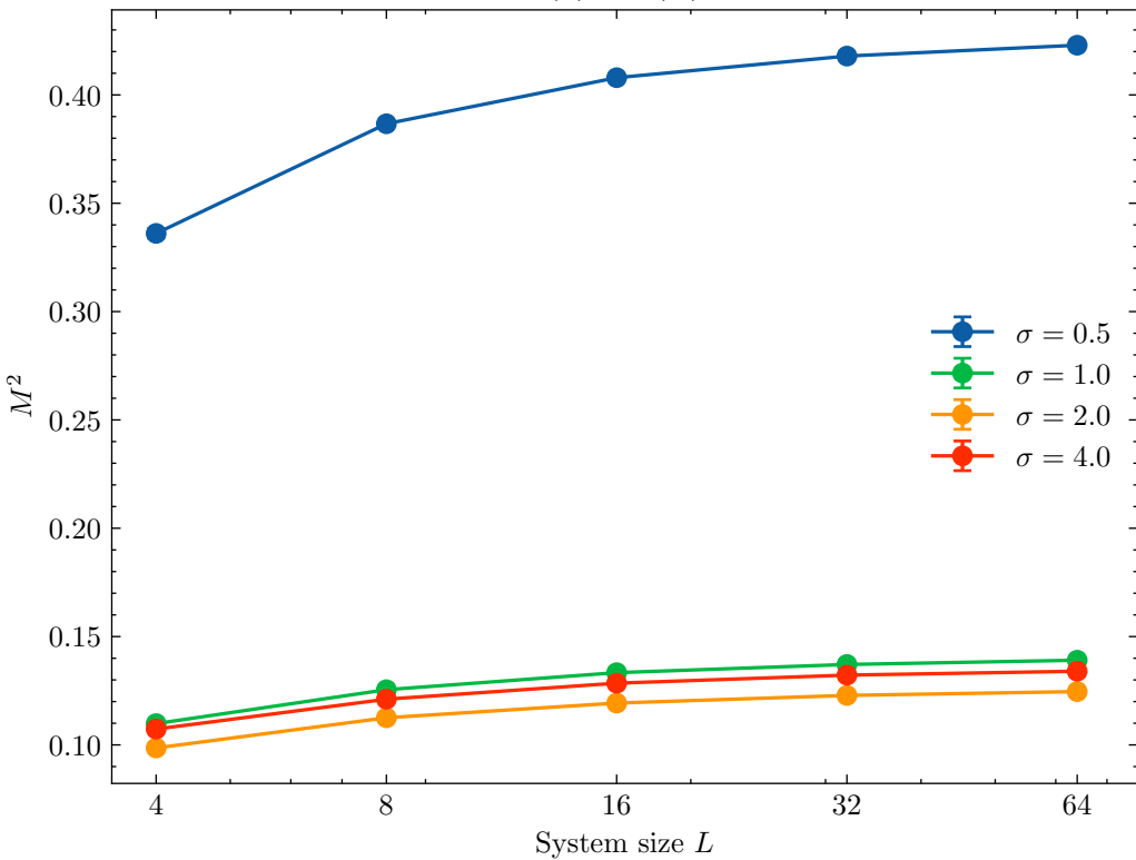
(a) M^2(L)
