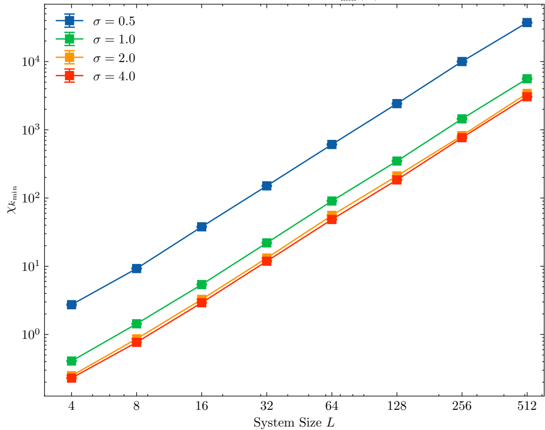
Structure Factor \chi_{k_{\min}}(L)
