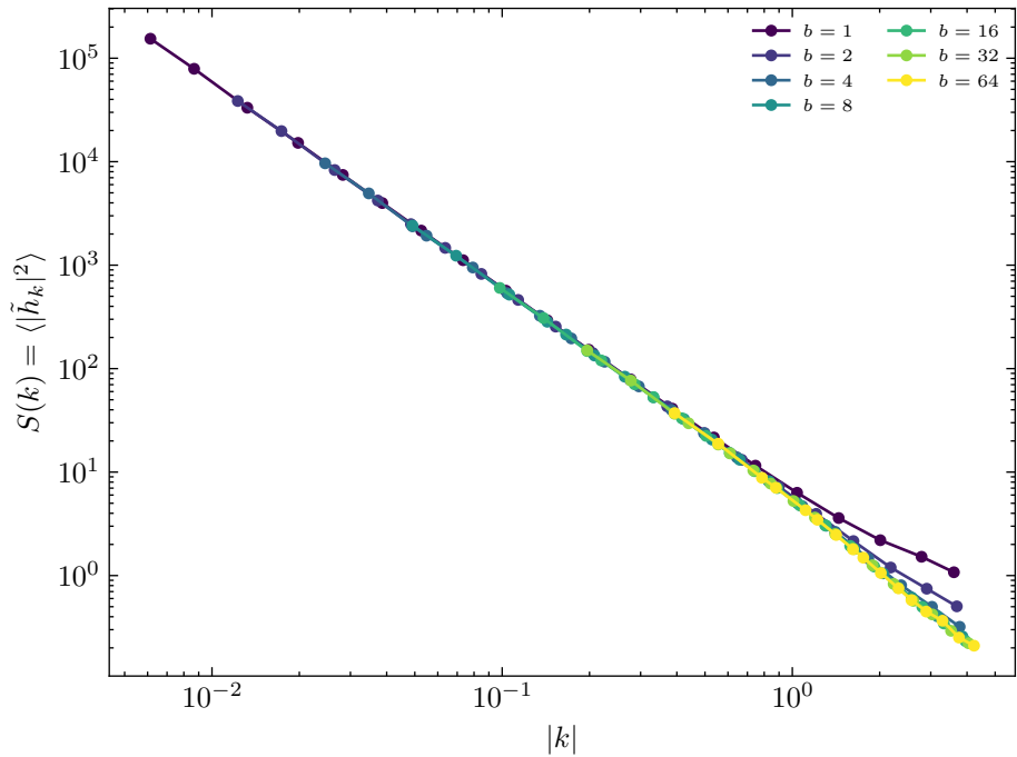
Structure factor S(k) ( L = 1024 , \sigma = 0.5 )
