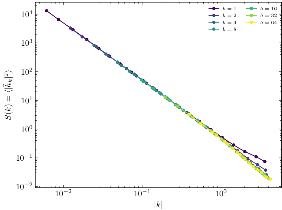
Structure factor S(k) ( L = 1024 , \sigma = 2.0 )
