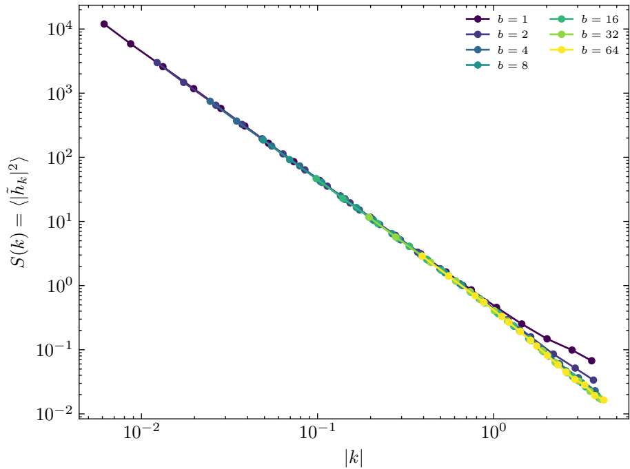
Structure factor S(k) ( L = 1024 , \sigma = 4.0 )
