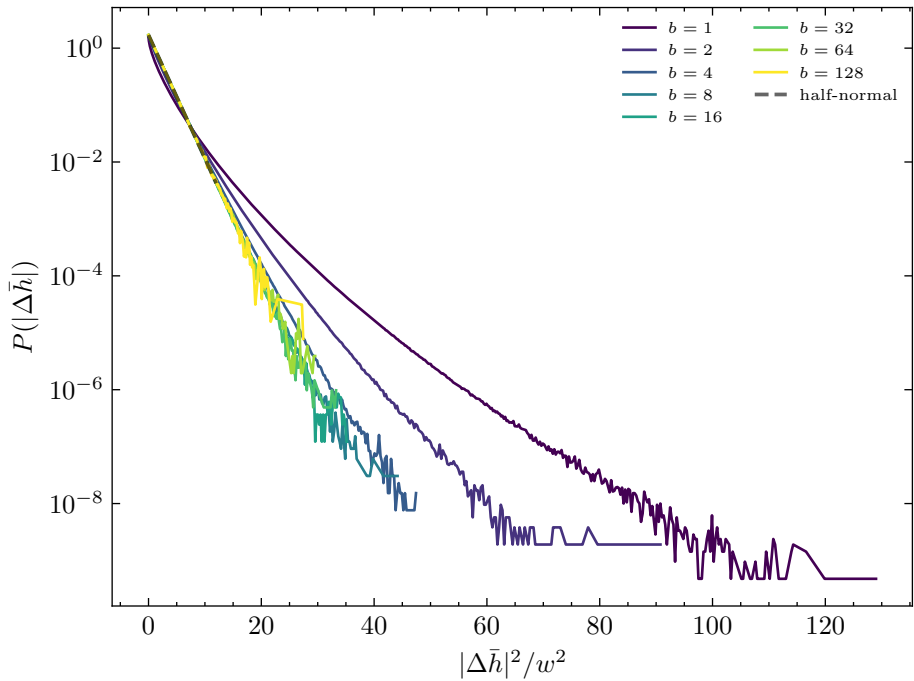
Height diff. distribution ( L = 1024 , \sigma = 1.0 )
