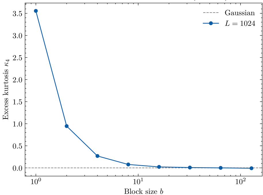
Excess kurtosis \kappa_4 vs block size b ( \sigma = 0.5 )
