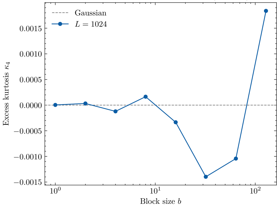
Excess kurtosis \kappa_4 vs block size b ( \sigma = 2.0 )
