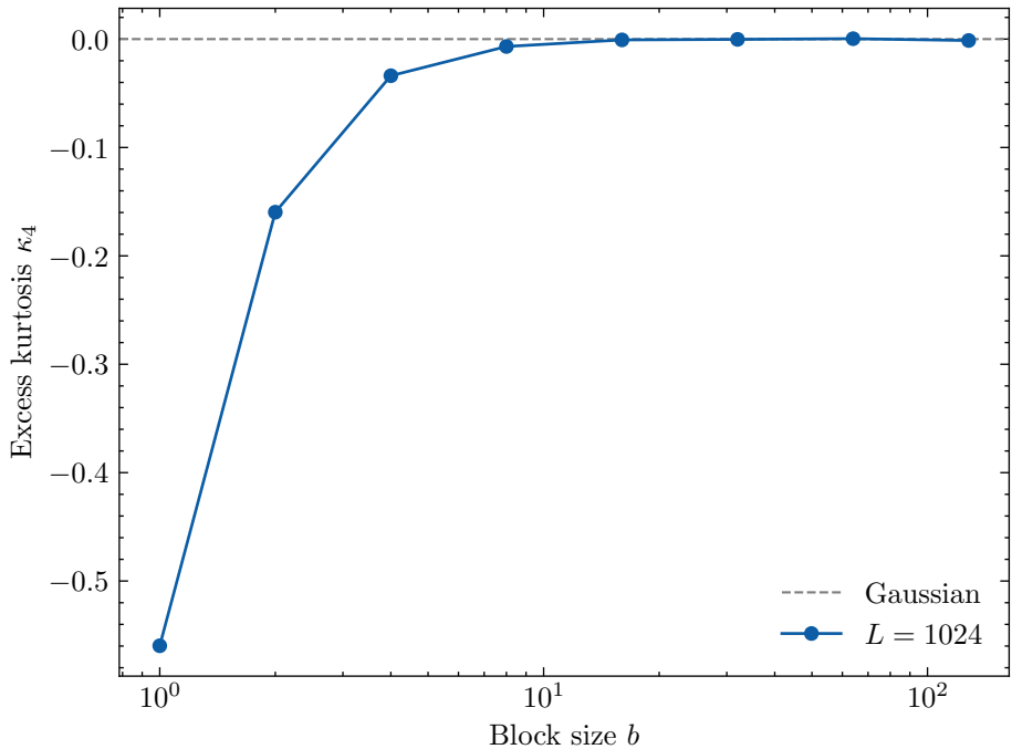
Excess kurtosis \kappa_4 vs block size b ( \sigma = 4.0 )
